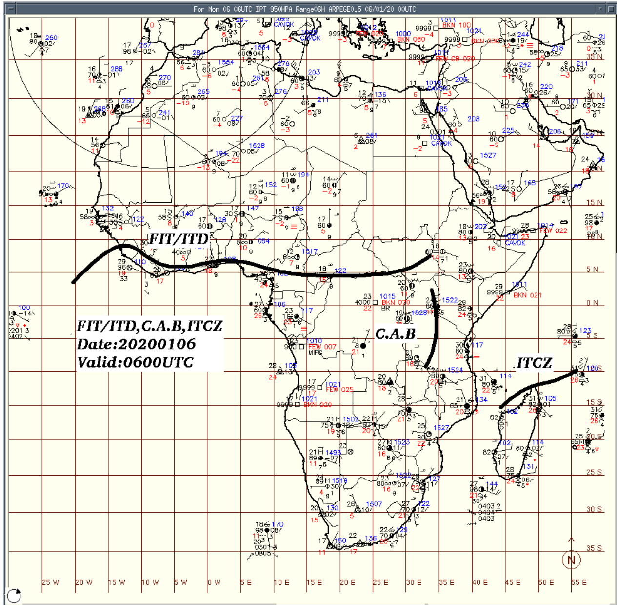
Tabulated positions of the ITD: 06 th JANUARY 2020
